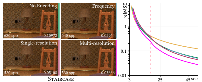
Figure 8: Equal-time comparison (50s) of different input encoding. We report the sample count and error (relMSE) of each method. The dashed line in the plot marks the end of the training phase. The multi-resolution spatial embedding outperforms other methods while remaining training-efficient. Yellow plot refers to path tracing with BxDF importance sampling.
