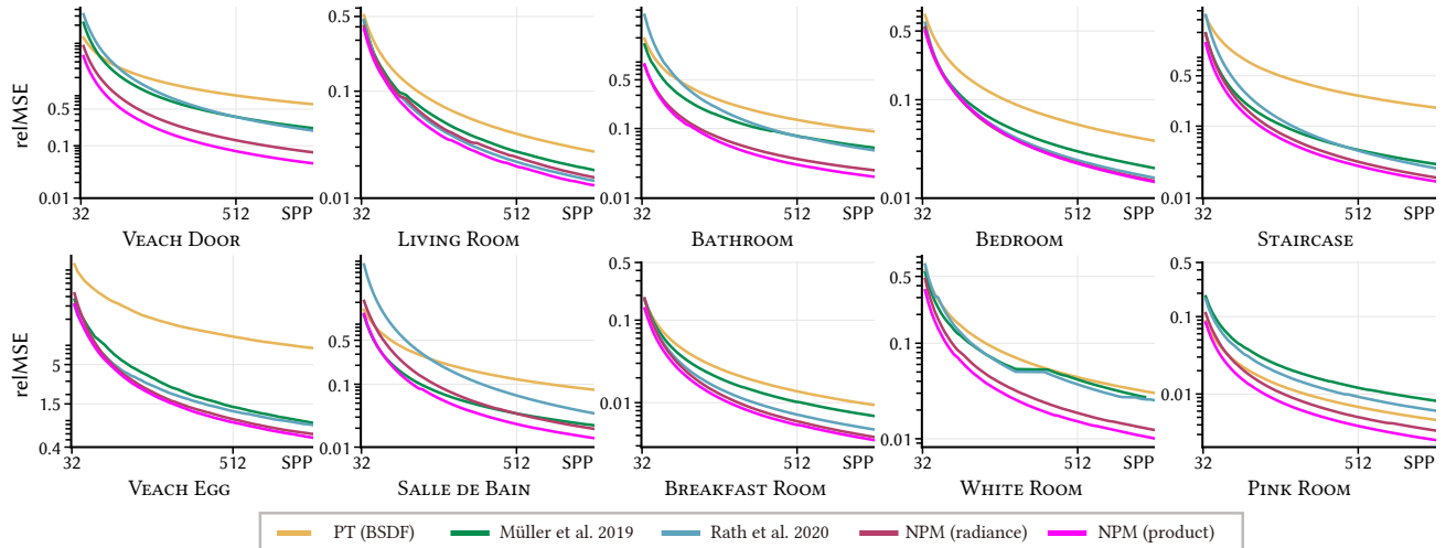
Figure 5: Convergence plots correspond to Fig. 3 and Fig. 4. Unidirectional path tracing with BxDF importance sampling (PT-BSDF), Practical Path Guiding [Müller 2019], Variance-aware Path Guiding [Rath et al. 2020] and our method with different target distributions (NPM-radiance and NPM-product). Our methods consistently outperform these classical guiding methods, and quickly become effective even with a few training samples and short training time (e.g., 30spp, amounting to about 3 seconds on GPU), indicating practicality for preview or even interactive rendering. We attribute this success to the compact implicit representation and better spatial resolution of our method. The image results and detailed statistics could be inspected in the supplemental materials.
