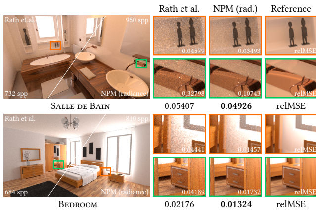
Figure 6: Equal-time comparisons (80s) on two test scenes between NPM(radiance) and Variance-aware Path Guiding [Rath et al. 2020].
