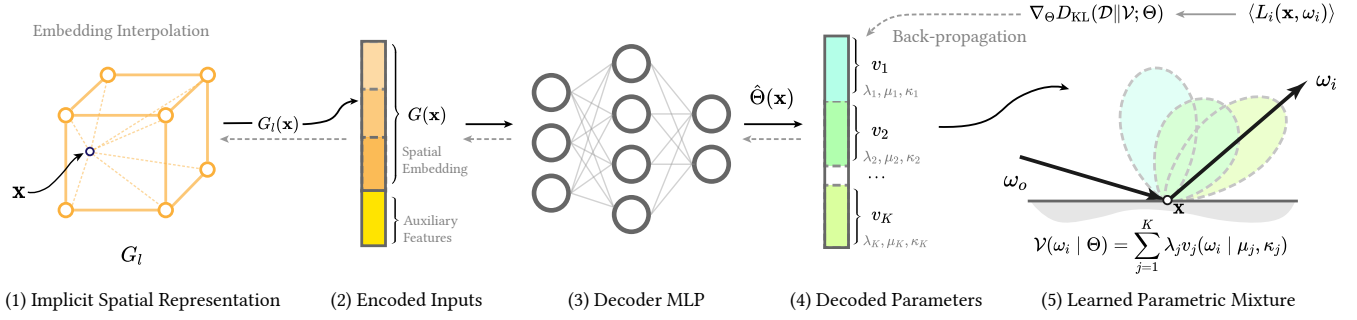
Figure 2: High-level illustration of our Neural Parametric Mixtures (NPM). We implicitly encode the spatially varying target distributions with the multi-resolution embedding. When the distribution of a spatial location \mathbf{x} is queried, (1) the features assigned to the nearby grid points surrounding \mathbf{x} are interpolated at each level, and concatenated with other levels to obtain the spatial embedding G(\mathbf{x}) . (2) the spatial embedding is then combined with other inputs to (3) feed into the lightweight MLP for (4) decoding the parameters \Theta of the vMF mixture \mathcal{V}(\omega_i | \Theta) with K components. We then (5) use this parametric distribution for importance sampling the scattering direction. The result MC radiance estimate \langle L_i(\mathbf{x}, \omega_i) \rangle is used to estimate the training gradient \nabla_{\Theta} D_{\text{KL}} (Sec. 4.2), which is then back-propagated through these differentiable stages to optimize our NPM representation (dashed lines).
