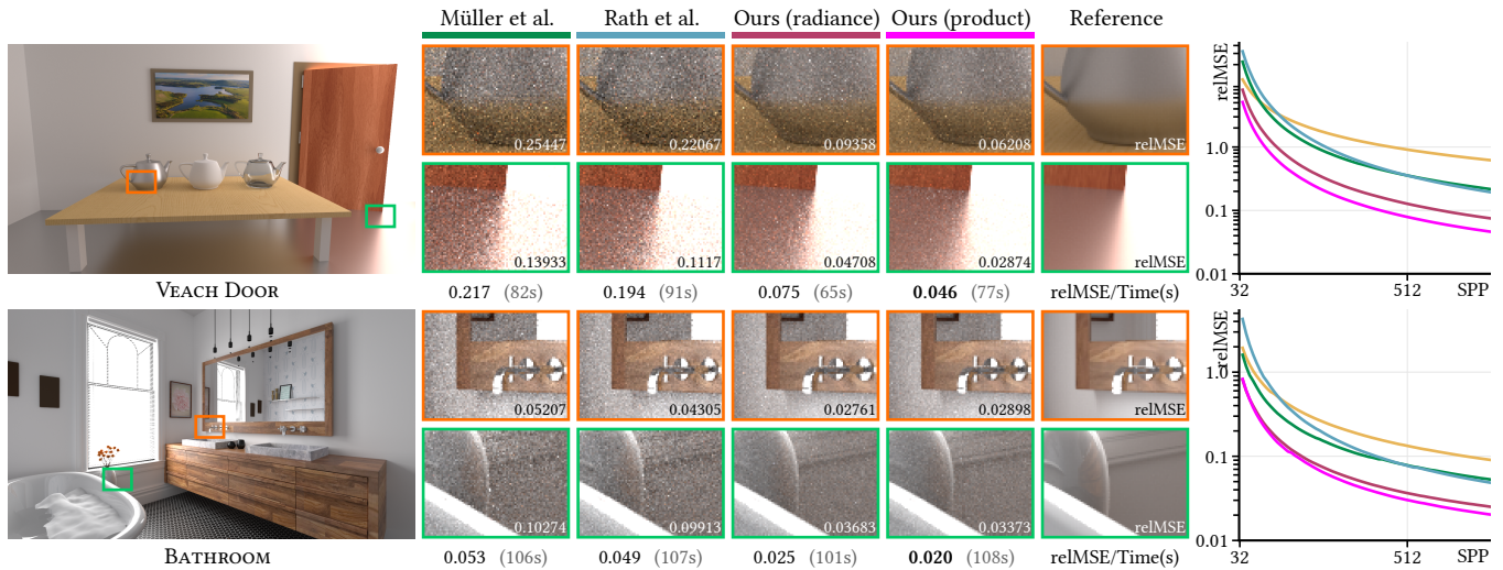
Figure 3: Equal-sample-count (750spp) comparisons for two scenes. We show the error (for both the zoom-in areas and whole images) and time cost of different methods. The yellow plots (as well as the other figures) refer to the results obtained by unidirectional path tracing.
