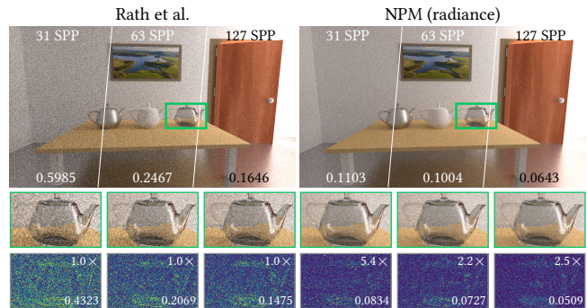
Figure 7: We train each guiding method with small training budgets (31 spp, 63 spp, 127 spp, respectively) and render the scene with 500 spp. Our method outperforms previous methods even with much fewer training samples.
