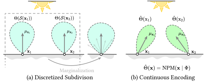
Figure 1: Parallax issue caused by spatial discretizations (a). For a subdivided volume \mathcal{S}(\mathbf{x}) in (a), the guiding distribution is marginalized with training samples scattered over the volume \mathcal{S}(\mathbf{x}) , and is shared by different positions (e.g., \mathbf{x}_1 and \mathbf{x}_2 ). Our method will not suffer from parallax due to NPM implicitly representing a monolithic function, continuously mapping from spatial positions to parametric guiding distributions, as shown in (b).
