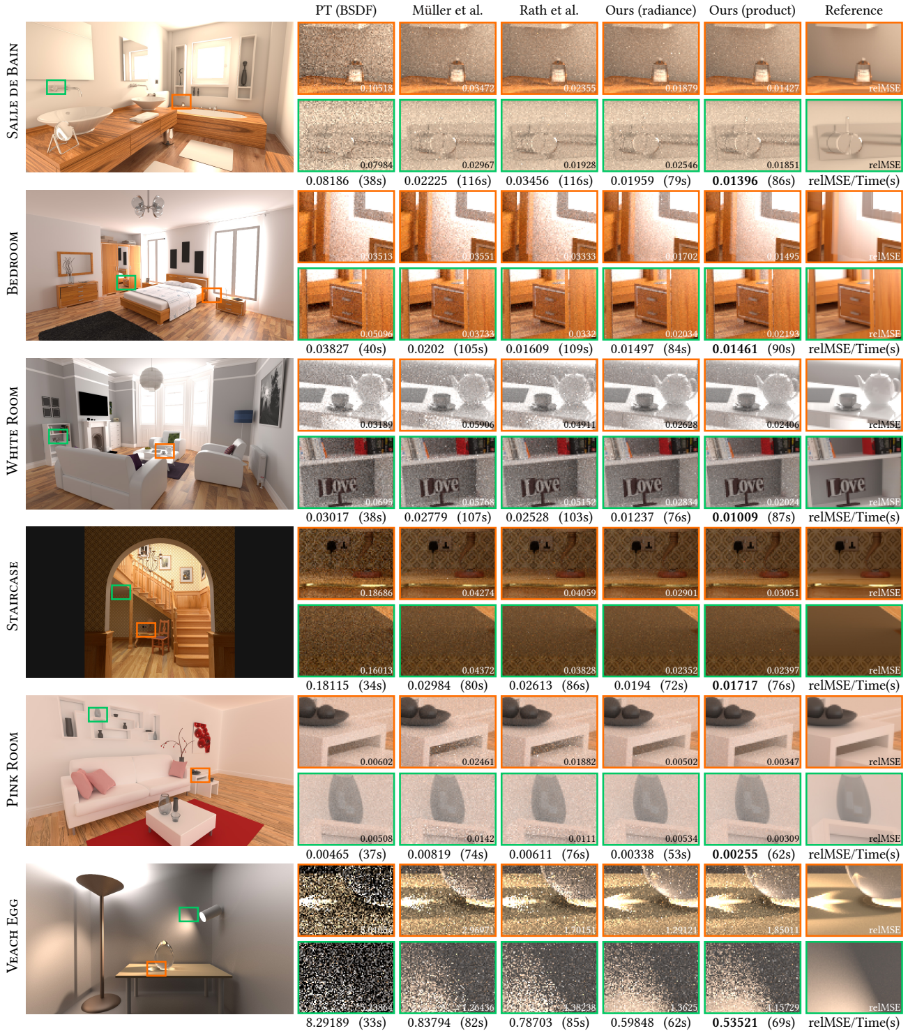
Figure 4: Visual comparisons using the same experimental setup with Fig. 3, all are rendered with 750 spp at 1280 × 720. We use the online training setup for all the guiding methods, i.e., all the samples are included in the final rendering. Our method exhibits better performance than other guiding methods in most scenes by only learning the incident radiance term while further reducing the error by incorporating the BSDF term (i.e., product sampling). More results on other test scenes, additional error metrics and false-color visualizations are provided in our supplementary interactive viewer.
